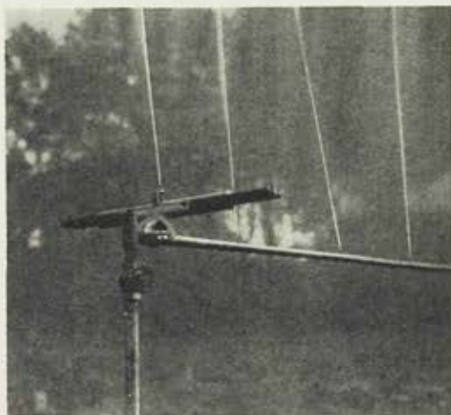
Fig. 2. Oscillator for rotating nozzle pipe on overhead pipe sprinkling irrigation system.
