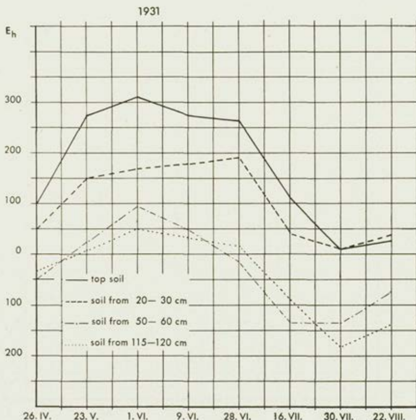
Diag. № 3. Redox-potential in the drained soil (under potatoes)
