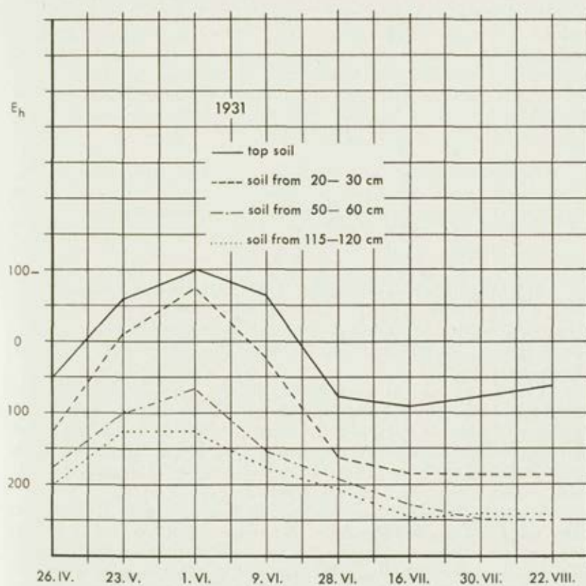
Diag. N° 4. Redox-potential in the undrained soil (under potatoes)
